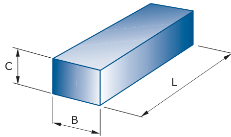
Honing stone Shape 5410 - B \times C \times L
